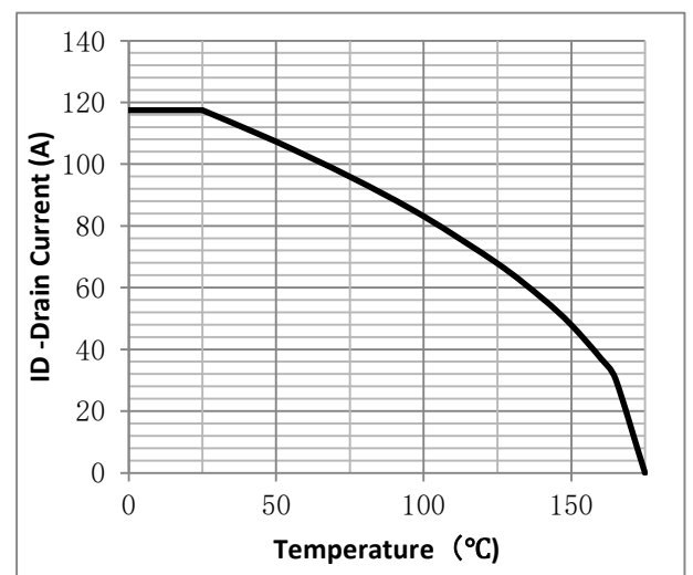
Fig.12 I_D vs. Junction Temperature②
